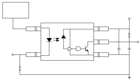
Fig.15: Test Circuit and Waveform of t_{PHL} , t_{PLH}
